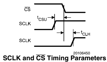
Serial Timing Diagram
