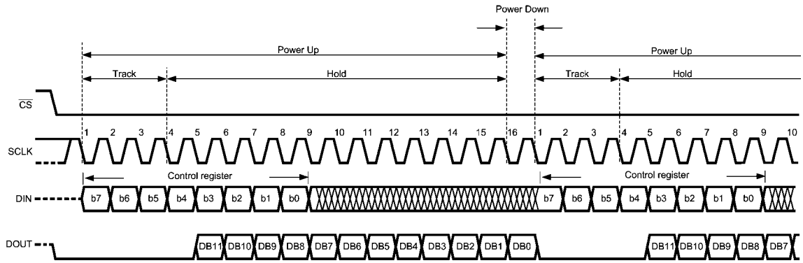
Operational Timing Diagram
