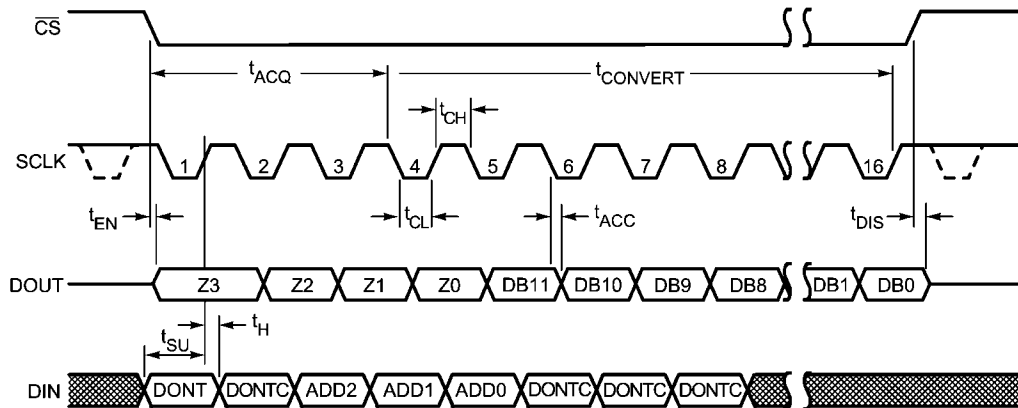
Serial Timing Diagram
